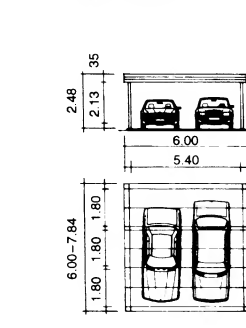
14 Double carports
